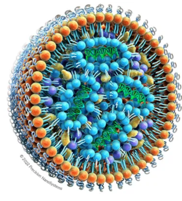
Lipid nanoparticle Delivery of mRNA
